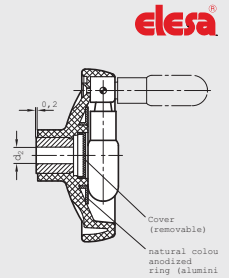
Elesa Model VDT+IR
