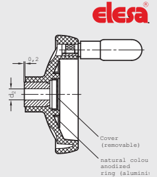
Elesa Model VDT, VDT+I
