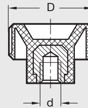
Elesa Model BT.S-INOX
