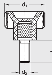
Elesa Model BT.p
