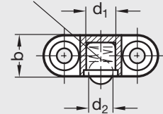
Spring plunger GN 614
